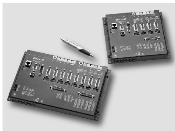
-BOX version of the DMC-41x3 controller
