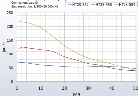
HT23-552/553/554, STAC6-220
