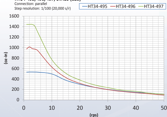
HT34-495/496/497, STAC6-220
