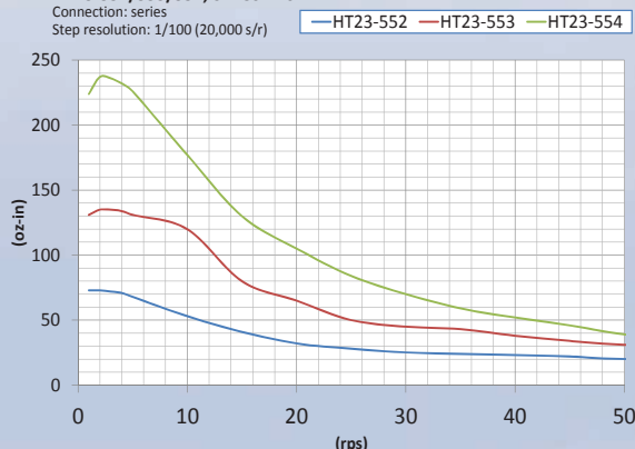
HT23-552/553/554, STAC6-220
