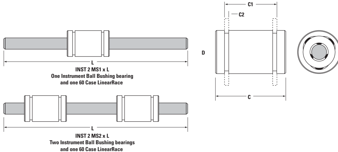
Miniature Instrument Ball Bushing Bearings and 60 Case LinearRace Sets (Dimensions in inches)
