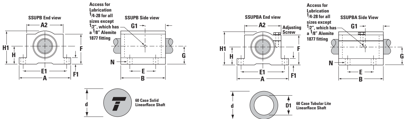
Super Smart Ball Bushing Pillow Blocks (Closed & Adjustable Types, seal at both ends) and LinearRace® (Dim. in inches)
