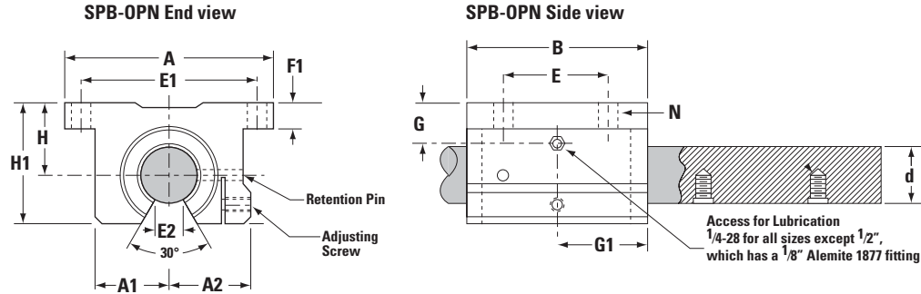
Super Ball Bushing Pillow Blocks (Open Type, seal at both ends) and 60 Case® LinearRace® (Dimensions in inches)
