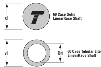
Sealed Super Ball Bushing Bearings (Closed Type, seal at both ends) and 60 Case® LinearRace® (Dimensions in inches)
