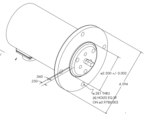
Fig. 9 Rugged Mount
