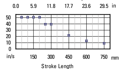
EC2-16B Ballscrew Critical Speed Limit
