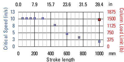
EC3-05B Ballscrew Specifications
