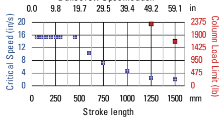
EC4-10B Ballscrew Specification
