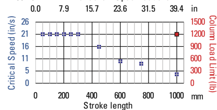
EC3-10B Ballscrew Specifications
