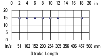
N2-5B Ballscrow Critical Speed Limit
