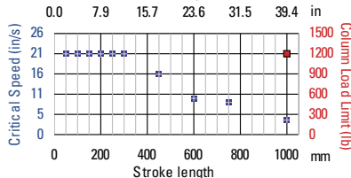
EC3-10B Ballscrew Specifications
