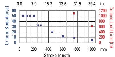
EC3-16B Ballscrew Specifications
