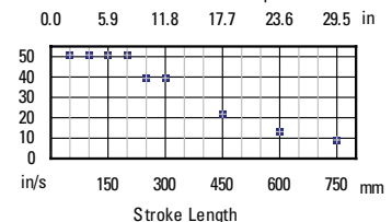
EC2-16B Ballscrew Critical Speed Limit
