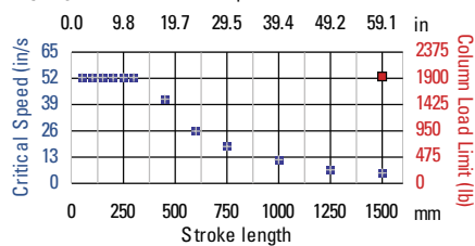
EC4-25B Ballscrew Specifications
