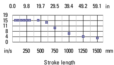
EC5-10B Ballcrew Critical Speed Limit
