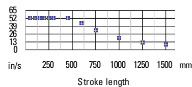
EC5-32B Ballscrew Critical Speed Limit
