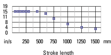
EC5-10B Ballscrew Critical Speed Limit
