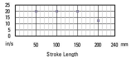
EC1-03M Ballscrew Critical Speed Limit
