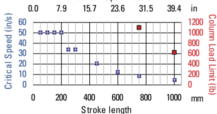
EC3-16B Ballscrew Specifications
