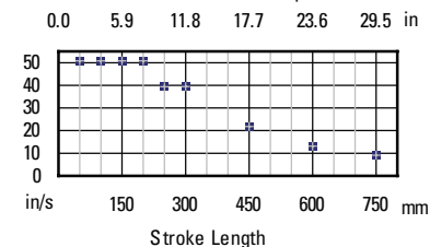
EC2-16B Ballscrew Critical Speed Limit
