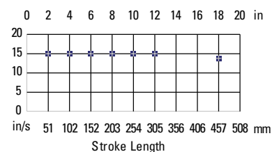
N2-5A Acme Screw Critical Speed Limit
