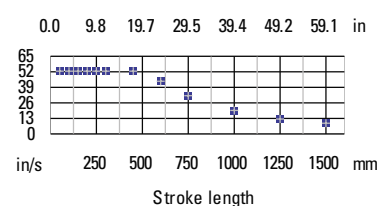
EC5-32B Ballcrew Critical Speed Limit
