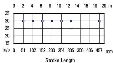
N2-2B Ballscrow Critical Speed Limit
