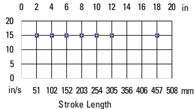
N2-5B Ballscrew Critical Speed Limit
