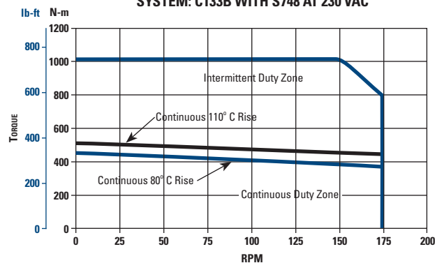
SYSTEM: C133B WITH S748 AT 230 VAC
