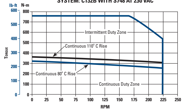
SYSTEM: C132B WITH S748 AT 230 VAC
