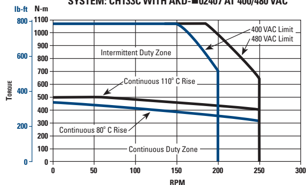
SYSTEM: CH133C WITH AKD-■02407 AT 400/480 VAC
