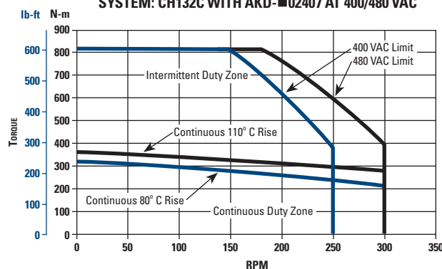
SYSTEM: CH132C WITH AKD-■02407 AT 400/480 VAC
