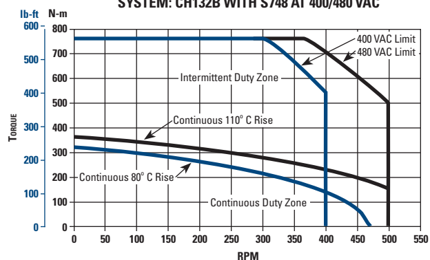
SYSTEM: CH132B WITH S748 AT 400/480 VAC
