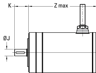
AKMH front mounting
