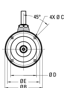
Open keyway (BK, CN, DK versions)
