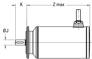
AKMH flange mounting
