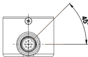
Position of M12 connector key
